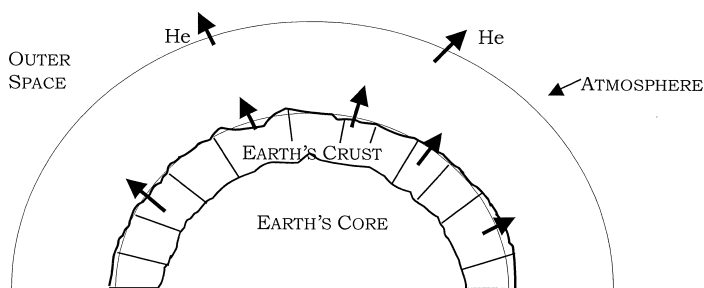
Figure 2. BUILD UP OF HELIUM IN THE EARTH'S ATMOSPHERE
