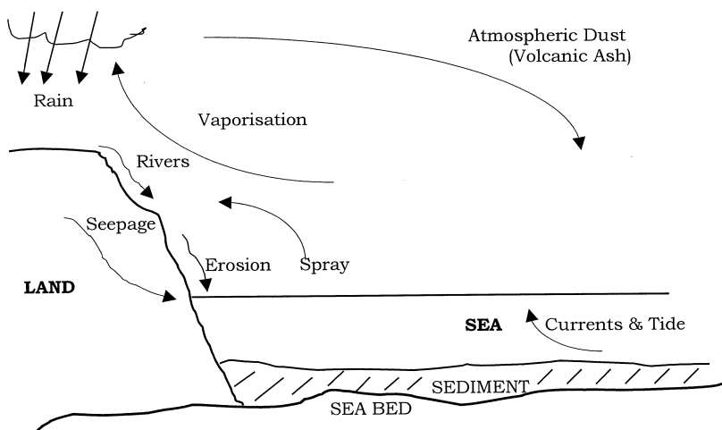
Figure 3. FACTORS THAT AFFECT THE SALTINESS OF THE SEA
