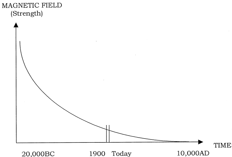
Figure 1. DECLINE OF THE EARTH'S MAGNETIC FIELD
